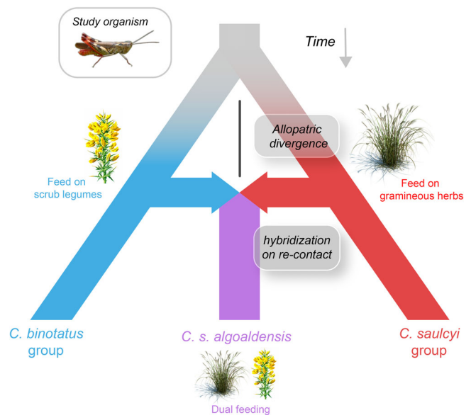
Figure 1. A graphical representation of the speciation history of C. s. algoaldensis inferred by the authors. Time runs down the page from a single common ancestor leading to the three contemporary groups. The initial divergence of the lineages leading to C. binotatus and C. saulcyi was facilitated by a period of geographic isolation (allopatry), which allowed feeding preferences to diverge. Upon secondary contact, hybridization led to the formation of a new lineage, ultimately giving rise to the dual-feeding C. s. algoaldensis .
